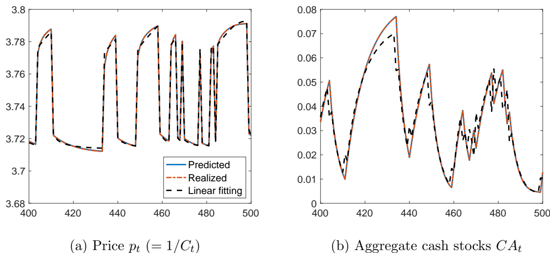
Figure 6: Aggregate fluctuations in the baseline model
